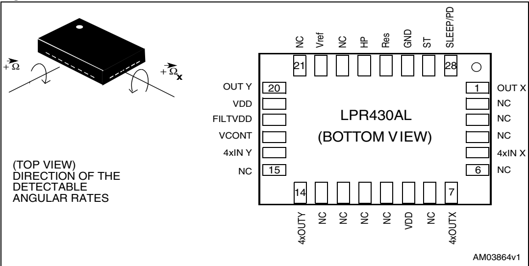
Figure 2. Pin connection
